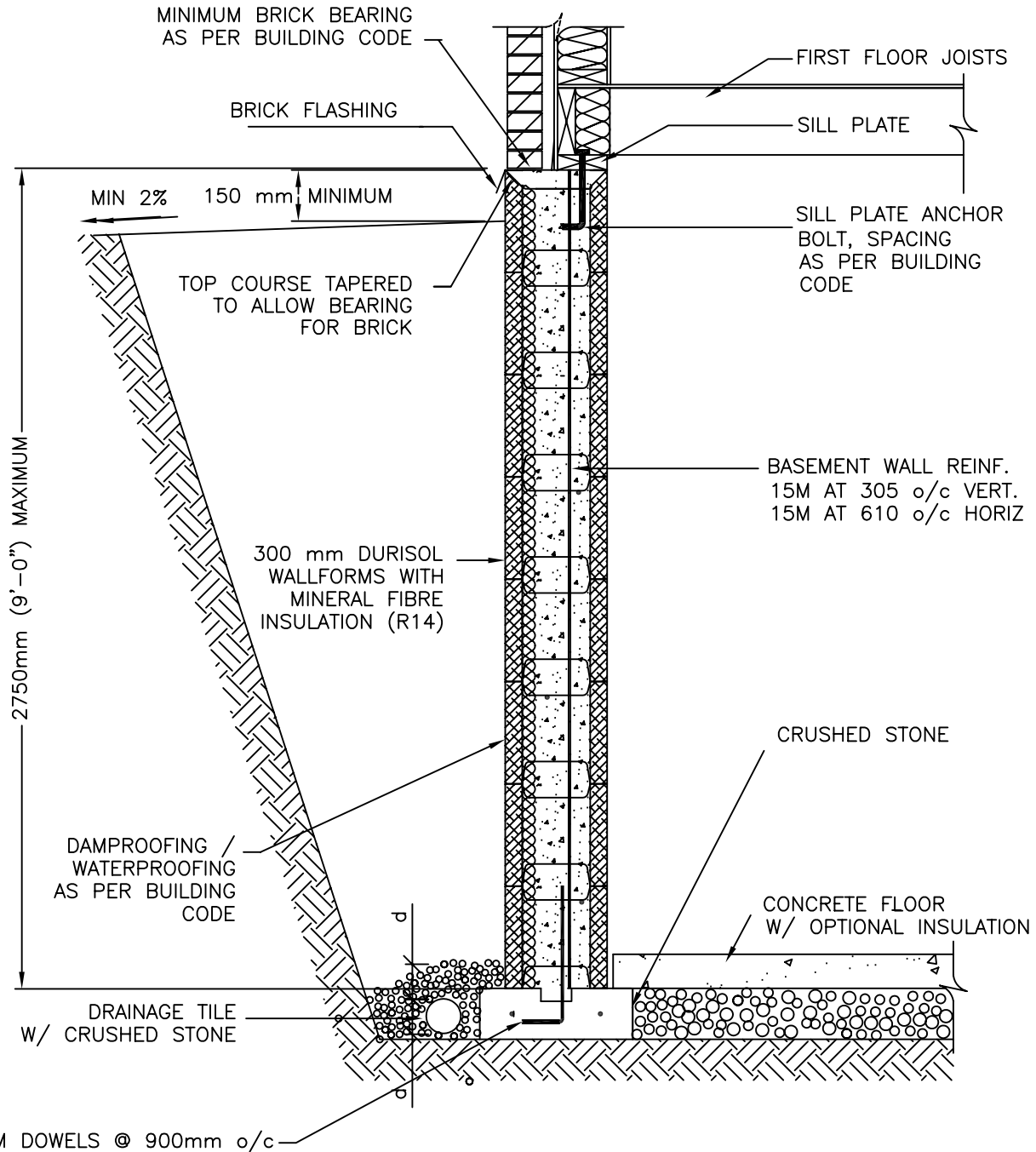
TYPICAL SECTION
