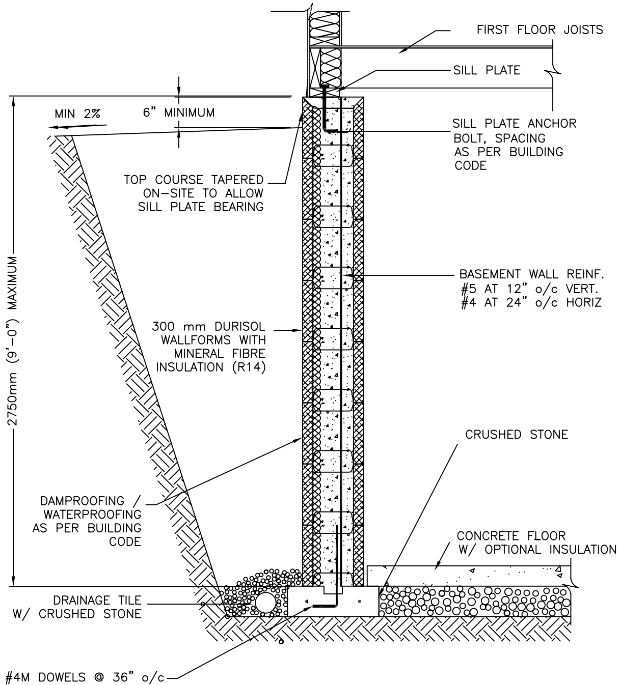
TYPICAL SECTION
