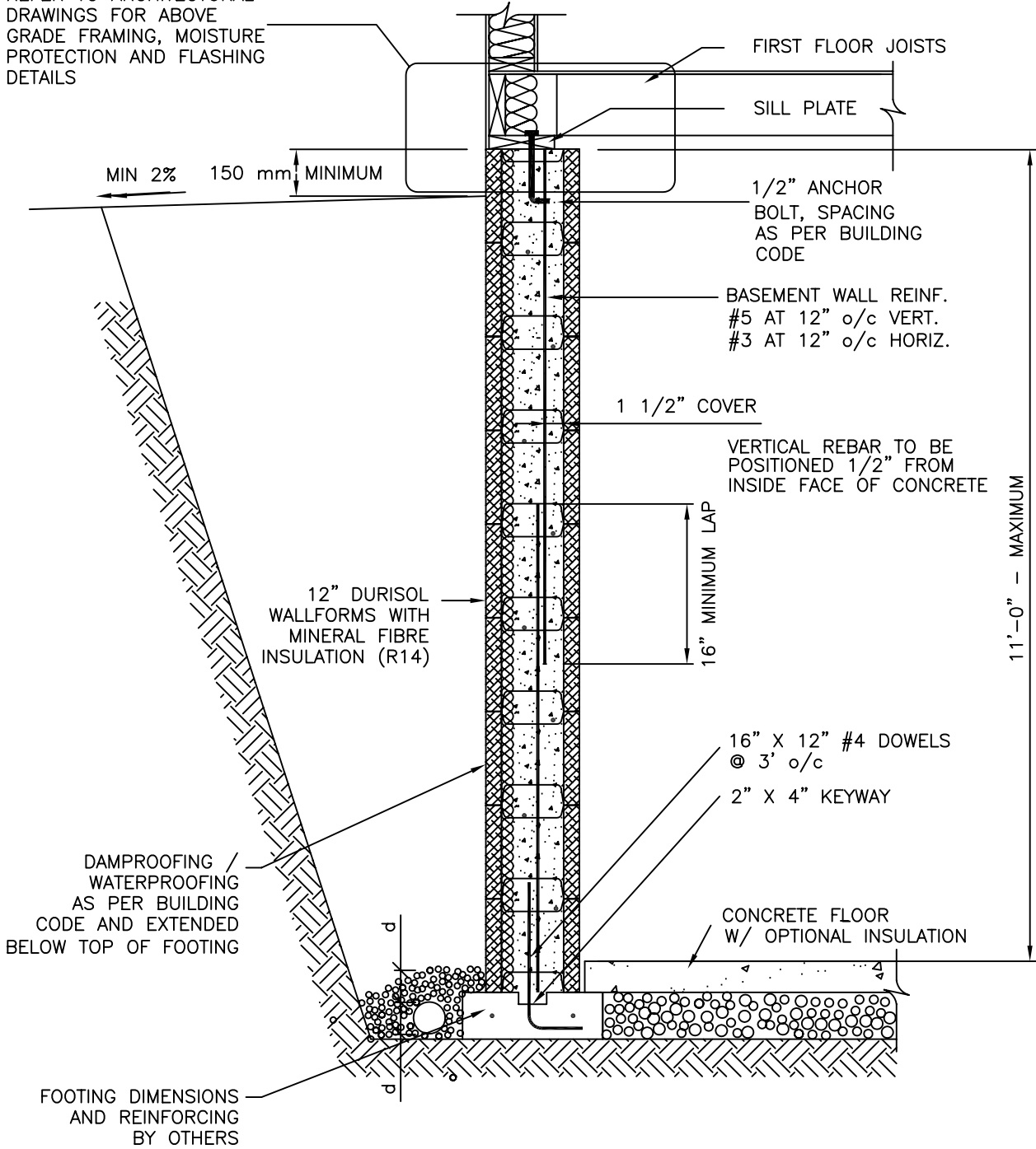
TYPICAL SECTION
